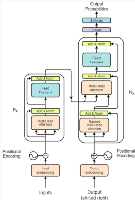
Figura 4: Attention Is All You Need
