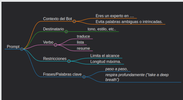
Figura 8: Resumen prompt
