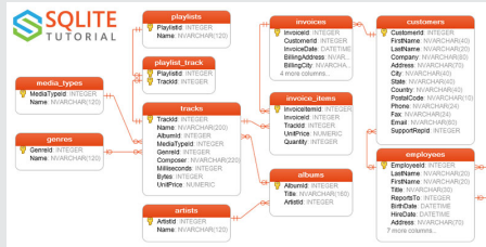
Figura 9: Chinook DB
